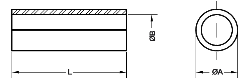
IT3420-XXA Neoprene Sleeve used with Class C Cable Clamps
