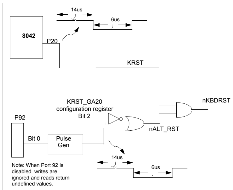
Figure 7.1 – NKBDRST Circuit
