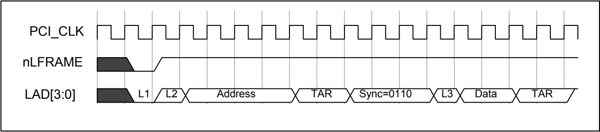
Figure 13.8 - I/O Read
