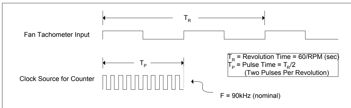
Figure 7.5 – Fan Tachometer Input and Clock Source
