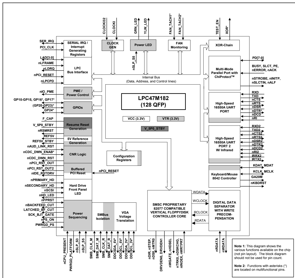
Figure 4.1 – LPC47M182 Block Diagram
