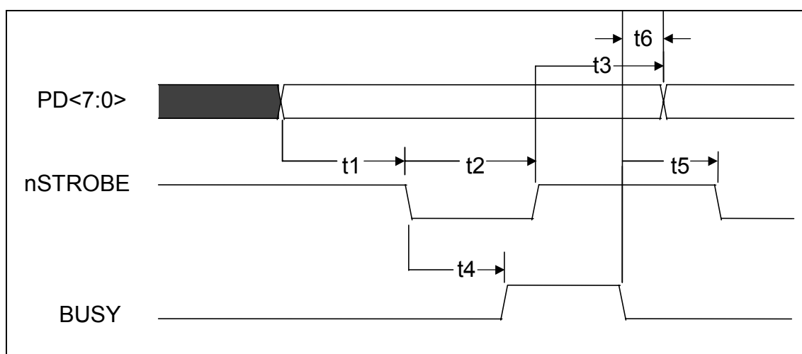
Figure 13.17 – Parallel Port FIFO Timing
