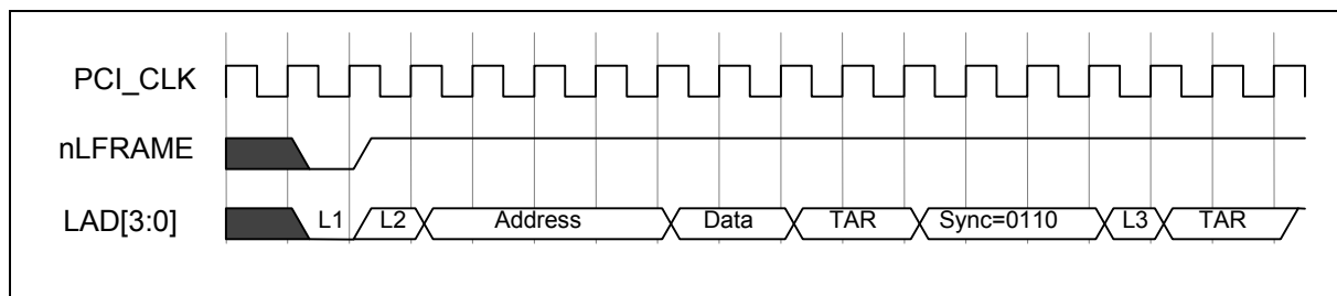
Figure 13.7 - I/O Write
