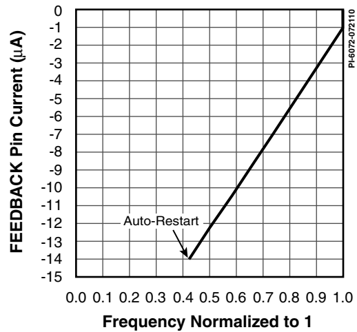
Figure 21. Frequency Cut Back in CC Mode Normalized to 1.
