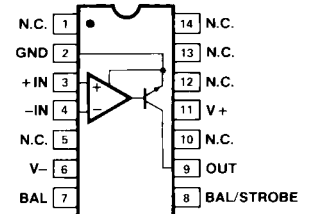
14-PIN HERMETIC DIP (Y-Suffix)
