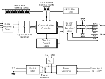
ADAM-4520 Converter Function Diagram
