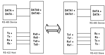
ADAM-4510/4510S Repeater Connection Diagram
