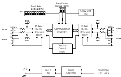
ADAM-4510 Repeater Function Diagram
