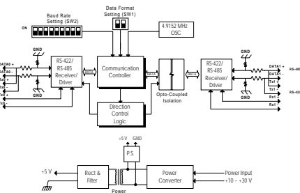
ADAM-4510S Repeater Function Diagram
