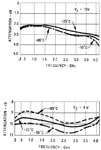
Attenuation vs. V_{CONTROL} vs. Frequency
