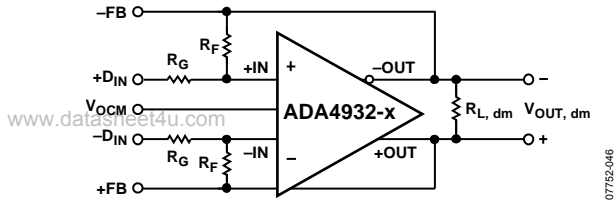
Figure 55. Signal and Circuit Definitions
