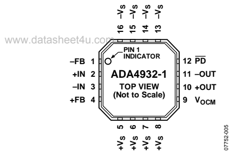
Figure 5. ADA4932-1 Pin Configuration
