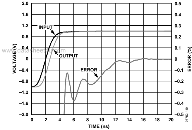
Figure 49. Settling Time
