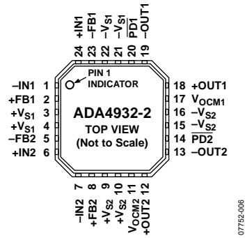
Figure 6. ADA4932-2 Pin Configuration
