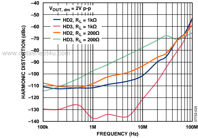
Figure 25. Harmonic Distortion vs. Frequency at Various Loads
