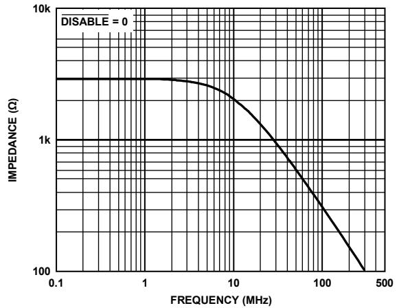
Figure 14. Output Impedance (Disabled) vs. Frequency
