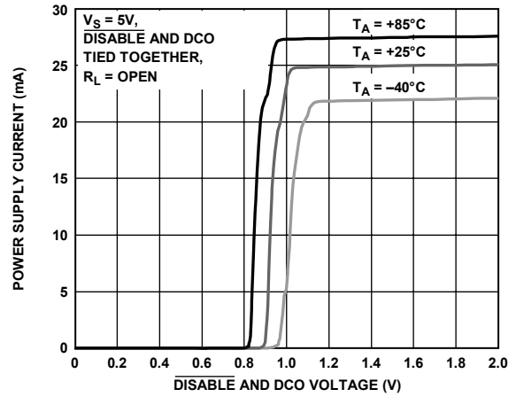
Figure 24. Supply Current vs. \overline{\text{DISABLE}}/\text{DCO} Voltage and Temperature
