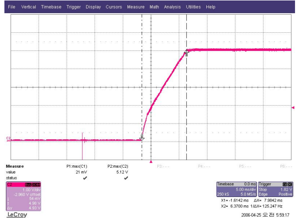
SFS5-5 7.98ms
