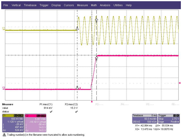
SFS5-24 32.9mS
