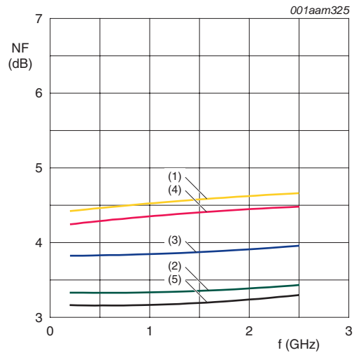
001aam325 Z_0 = 50 \Omega. (1) V_{CC} = 4.5 \text{ V}; T_{amb} = 85 \text{ }^\circ\text{C}; I_{CC} = 14.36 \text{ mA} (2) V_{CC} = 4.5 \text{ V}; T_{amb} = -40 \text{ }^\circ\text{C}; I_{CC} = 16.41 \text{ mA} (3) V_{CC} = 5.0 \text{ V}; T_{amb} = 25 \text{ }^\circ\text{C}; I_{CC} = 16.63 \text{ mA} (4) V_{CC} = 5.5 \text{ V}; T_{amb} = 85 \text{ }^\circ\text{C}; I_{CC} = 17.27 \text{ mA} (5) V_{CC} = 5.5 \text{ V}; T_{amb} = -40 \text{ }^\circ\text{C}; I_{CC} = 19.29 \text{ mA}
