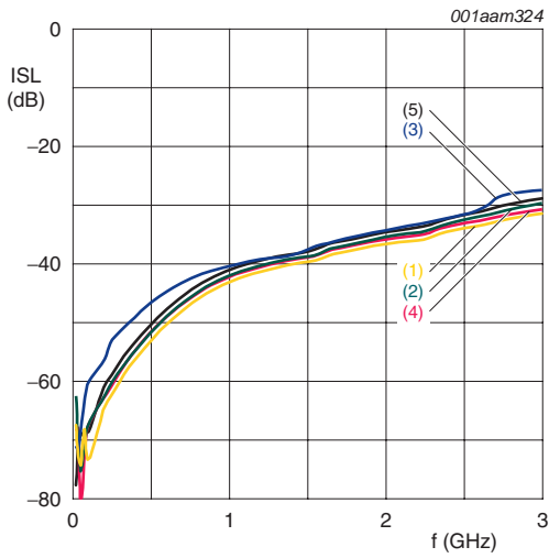
001aam324 P_{drive} = -40 \text{ dBm}; Z_0 = 50 \Omega. (1) V_{CC} = 4.5 \text{ V}; T_{amb} = 85 \text{ }^\circ\text{C}; I_{CC} = 14.36 \text{ mA} (2) V_{CC} = 4.5 \text{ V}; T_{amb} = -40 \text{ }^\circ\text{C}; I_{CC} = 16.41 \text{ mA} (3) V_{CC} = 5.0 \text{ V}; T_{amb} = 25 \text{ }^\circ\text{C}; I_{CC} = 16.63 \text{ mA} (4) V_{CC} = 5.5 \text{ V}; T_{amb} = 85 \text{ }^\circ\text{C}; I_{CC} = 17.27 \text{ mA} (5) V_{CC} = 5.5 \text{ V}; T_{amb} = -40 \text{ }^\circ\text{C}; I_{CC} = 19.29 \text{ mA}
