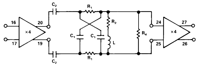
Figure 21. RLC Equalizer
