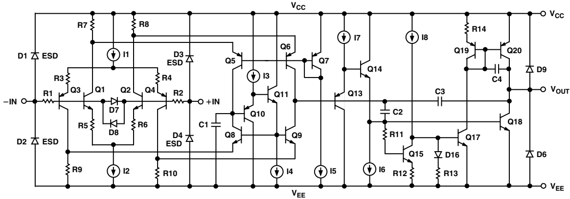
Figure 19. Simplified Schematic
