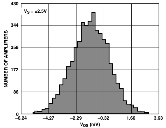
TPC 11. V_{OS} Distribution
