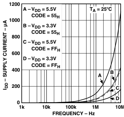
TPC 23. Supply Current vs. Clock Frequency
