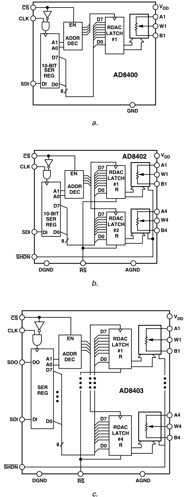
Figure 4. Block Diagrams
