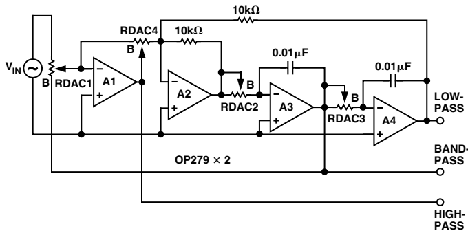
Figure 10. Programmable State Variable Active Filter
