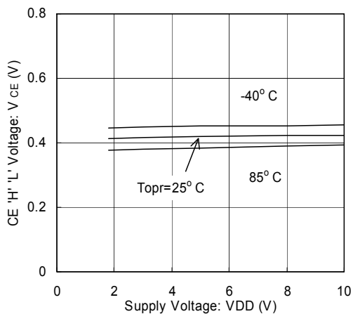
(8) CE 'H' 'L' Voltage vs. Supply Voltage
