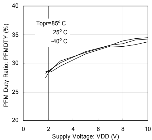
(18) PFM Duty Ratio vs. Supply Voltage
