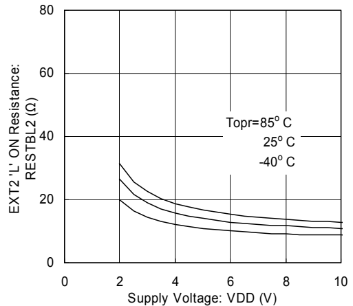
(15) EXT2 Low ON Resistance vs. Supply Voltage
