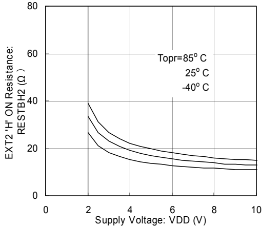
(14) EXT2 High ON Resistance vs. Supply Voltage
