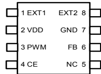
MSOP-8A (TOP VIEW)
