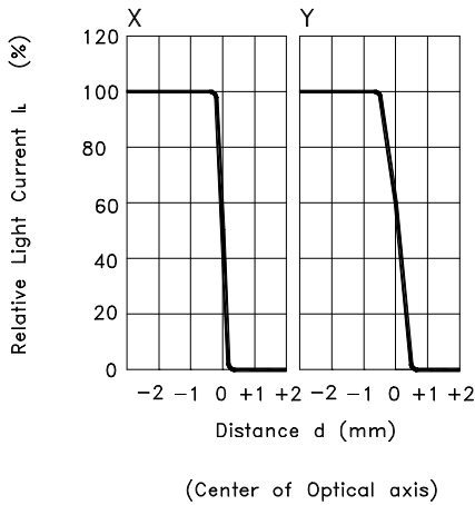
Fig.7 Sensing Position Characteristics (Typical)
