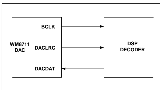
Figure 18 Master Mode
