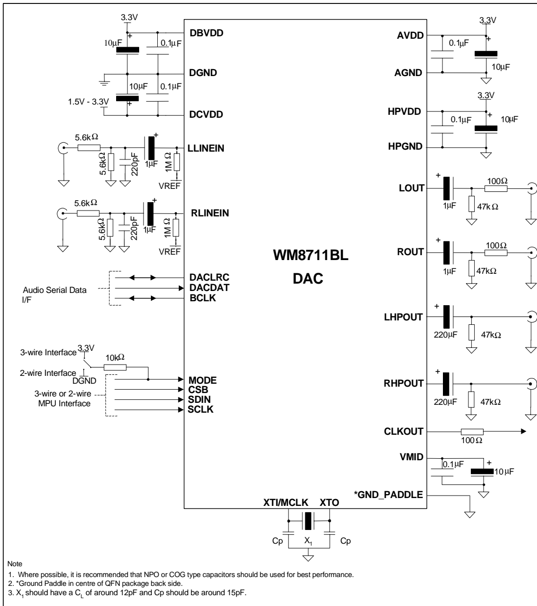
Figure 36 External Components Diagram
