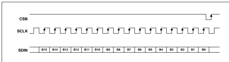
Figure 20 3-Wire Serial Interface
