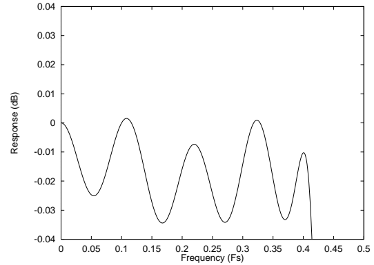
Figure 23 DAC Digital Filter Ripple-Type 0
