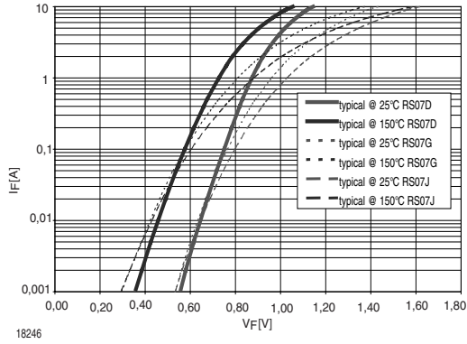
Figure 1. Typical Forward Characteristics
