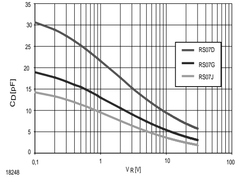
Figure 3. Typ. Diode Capacitance vs. Reverse Voltage
