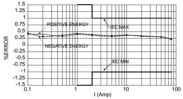
GRAPH 2 - Linearity PF=+0.5, FREQ=50Hz, Vnom, TEMP=25°C
