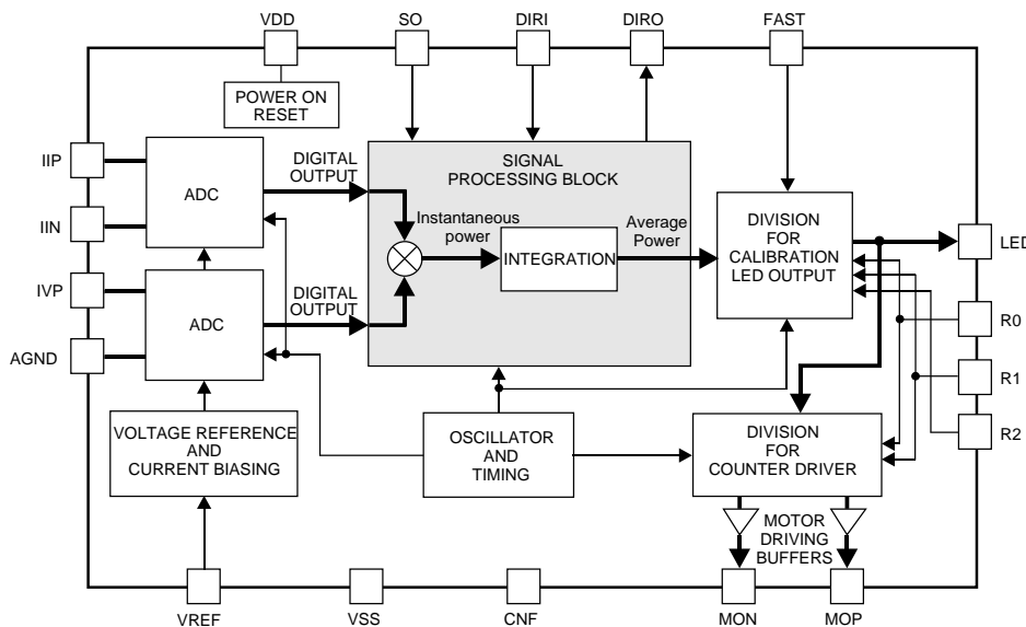
Figure 1: Block diagram
