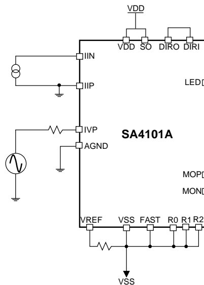
Figure 2: Test Circuit for Electrical Characteristics
