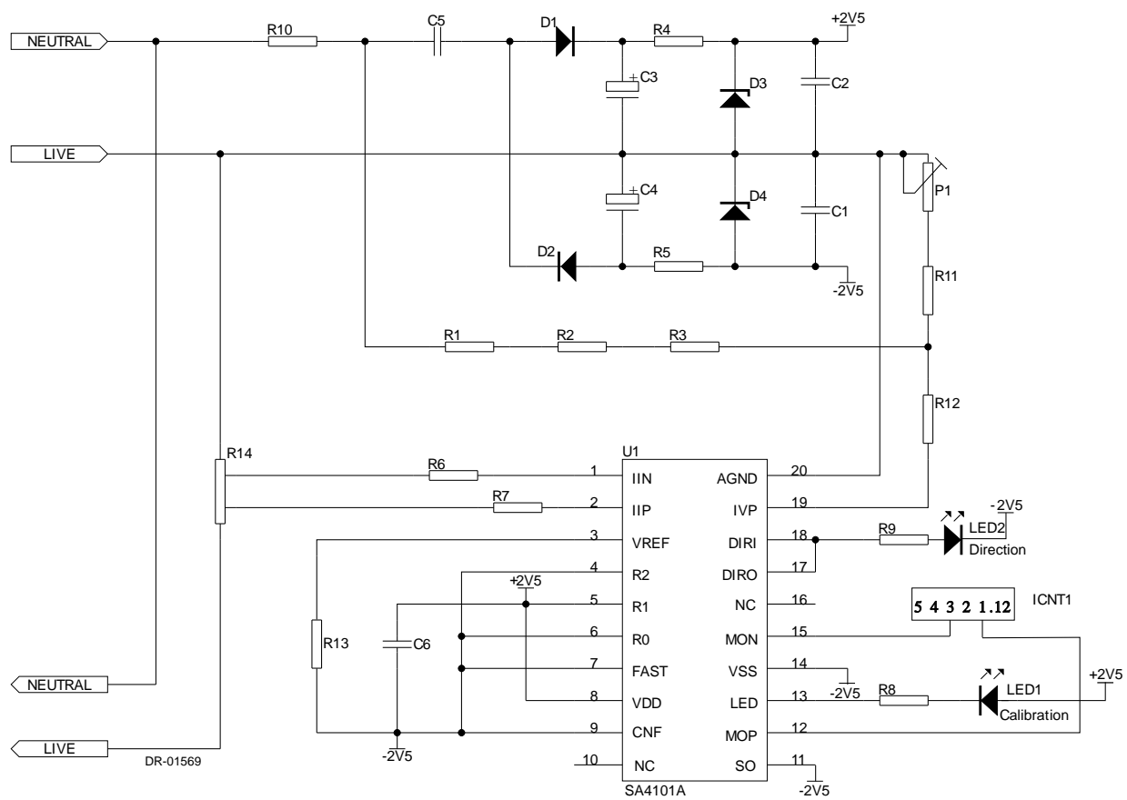
220V/40A meter with 1600 pulses/kWh resolution
