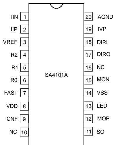
Figure 3: Pin connections: Package: PDIP20, SOIC20
