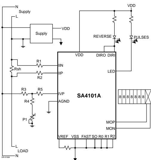
Figure 6: Application circuit
