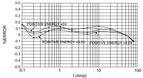
GRAPH 4 - Linearity PF=1, Supply=+5.5V, +5V, +4.5V
