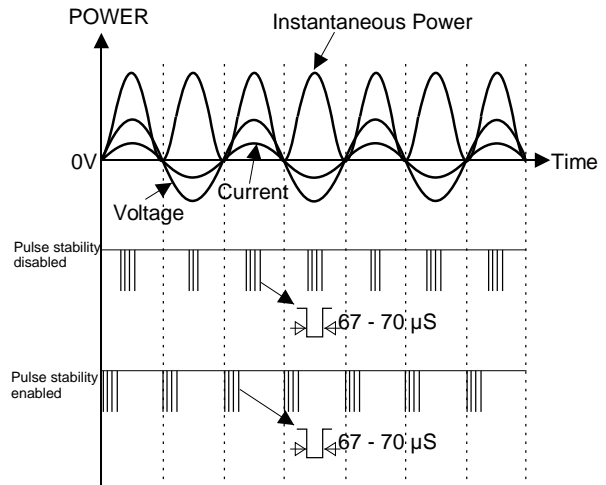
Figure 9: LED pulse output in fast mode
