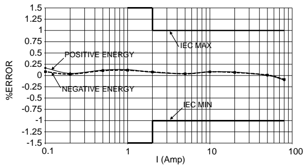
GRAPH 1 - Linearity PF=1, FREQ=50Hz, Vnom, TEMP=25°C
