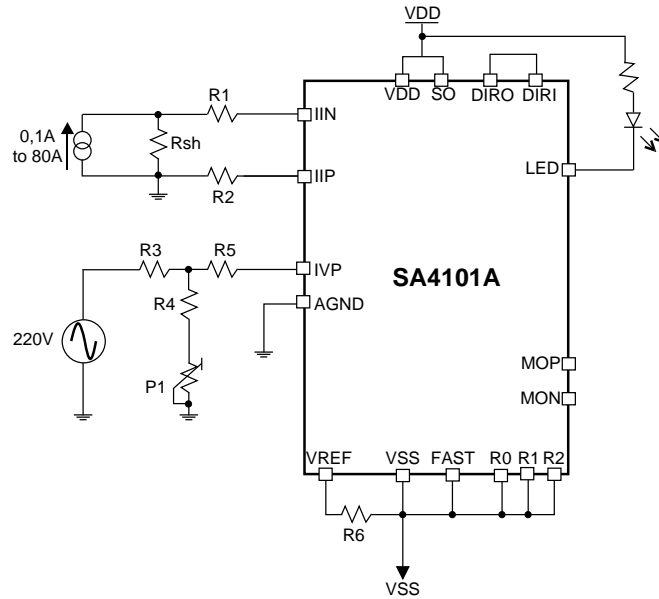
Figure 4: Test circuit for performance graphs
