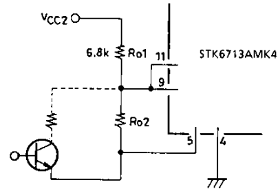
Fig. 4 Vref Peripheral Circuit
