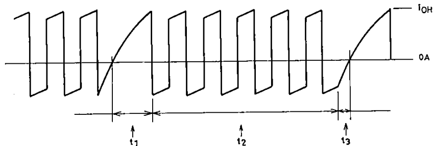
Fig. 7 Motor Output Current Waveform (model)
