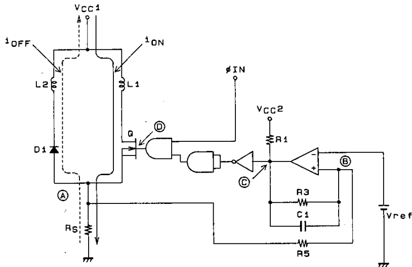
STK6713AMK4 Basic Circuit
