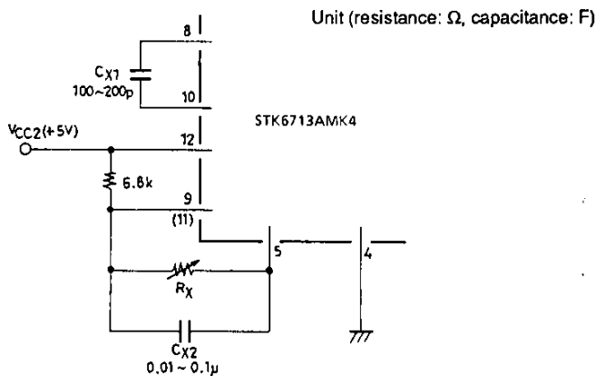
Fig. 10 Motor Hold Noise Countermeasure
