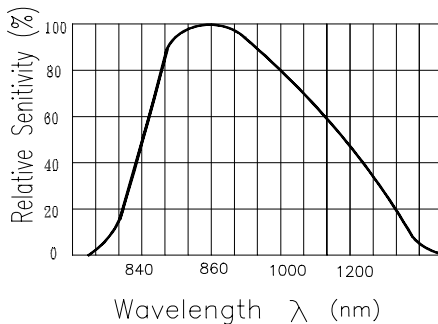
Fig.5 Spectral Sensitivity
