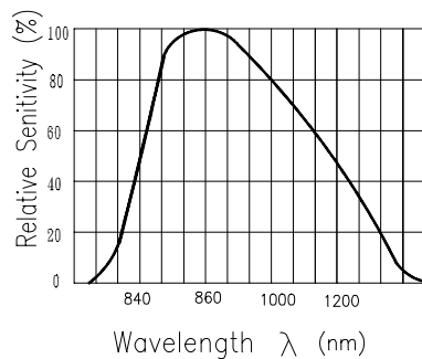
Fig.5 Spectral Sensitivity
