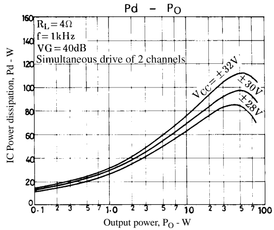
Figure 2. STK4181V Pd - P O (R L = 4Ω)
