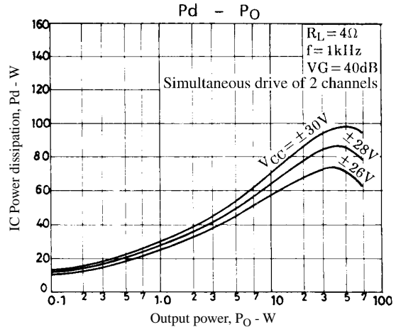
Figure 2. STK4171V Pd - P O (R L = 4Ω)
