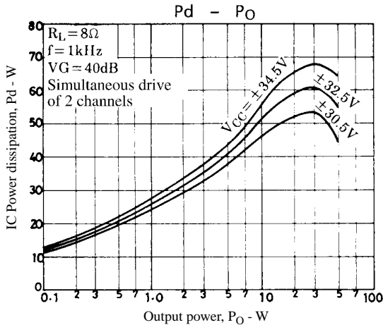
Figure 1. STK4171V Pd - P O (R L = 8Ω)
