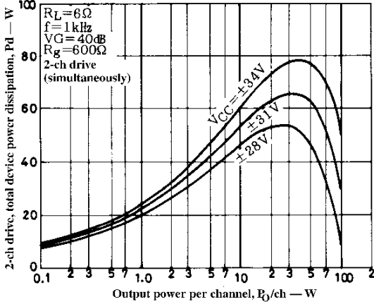
Figure 1. P_d - P_O
