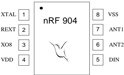
Figure 2. nRF904 pin assignment.
