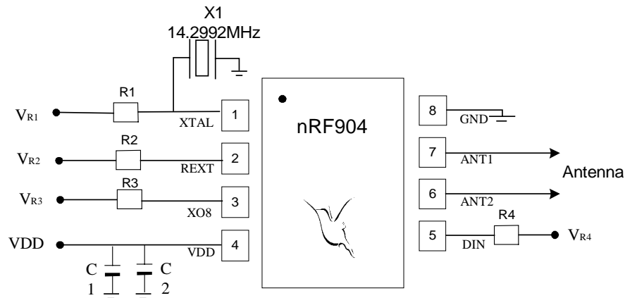
Figure 4. nRF904 with External Components.
