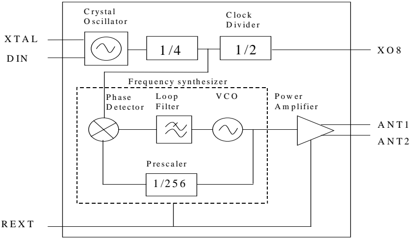
Figure 1. nRF904 block diagram.
