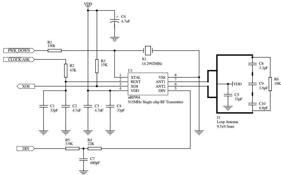
Figure 10. nRF904 application schematic.
