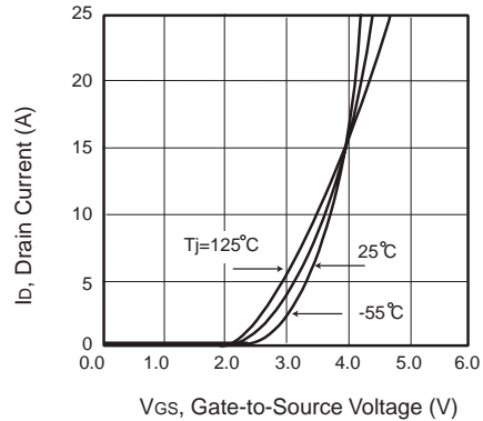
Figure 2. Transfer Characteristics
