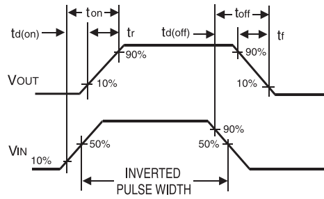
Figure 12. Switching Waveforms
