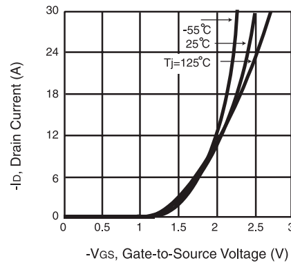
Figure 2. Transfer Characteristics
