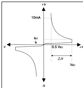
DIAGRAM 1: Current-voltage characteristics
