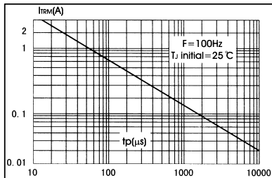
FIG.3-Peak pulse current versus pulse duration (maximum values)
