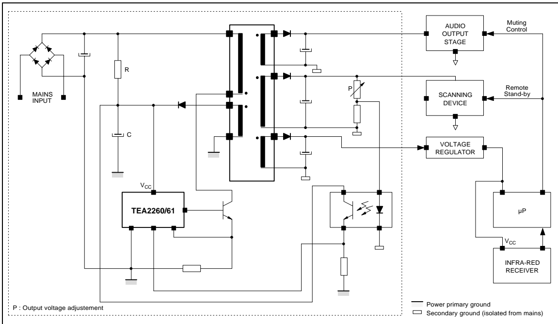
Figure 2 : Secondary Regulation (with optocoupler)
