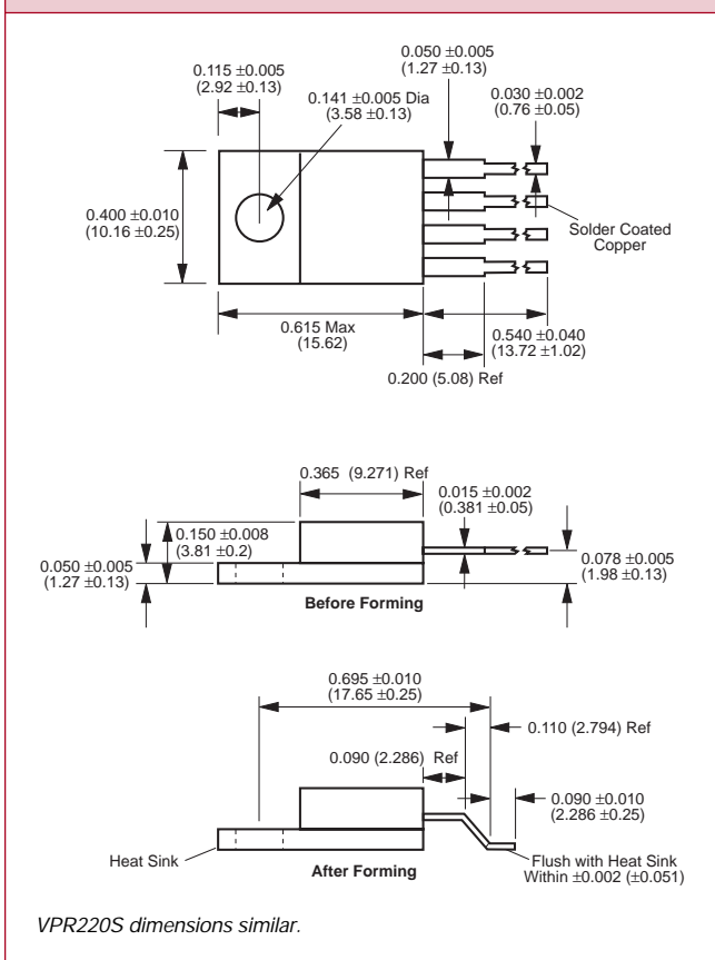
FIGURE 3 - VPR221S DIMENSIONS
