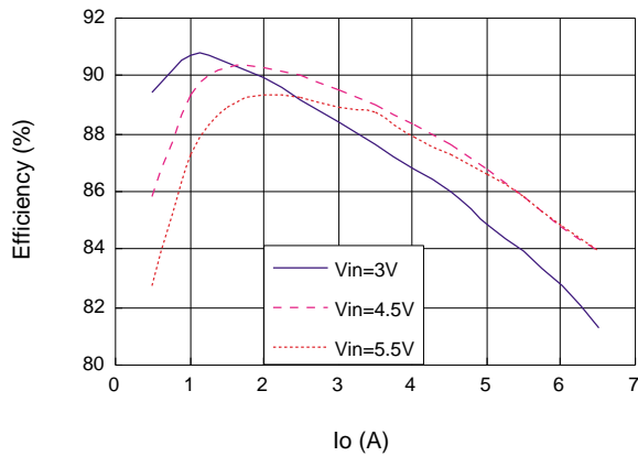
Typical Efficiency APA06G05(E-6)
