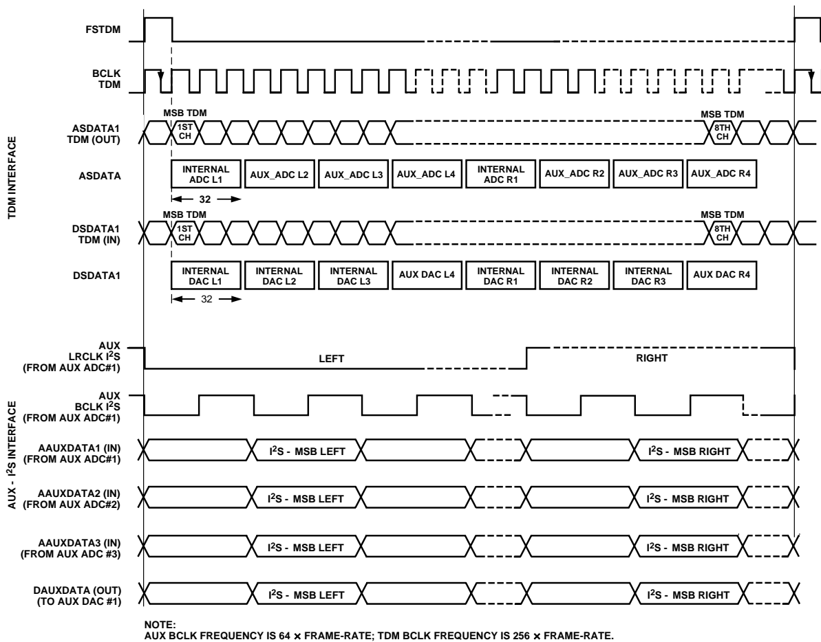
Figure 11. AUX-Mode Timing
