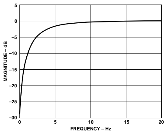
TPC 4. ADC High-Pass Filter Response, f_s = 96 \text{ kHz}
