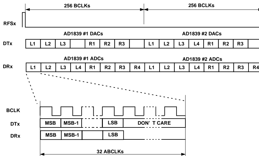
Figure 15. Cascade Timing
