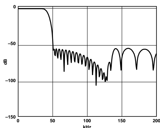
TPC 6. DAC Composite Filter Response, f_s = 96 \text{ kHz}
