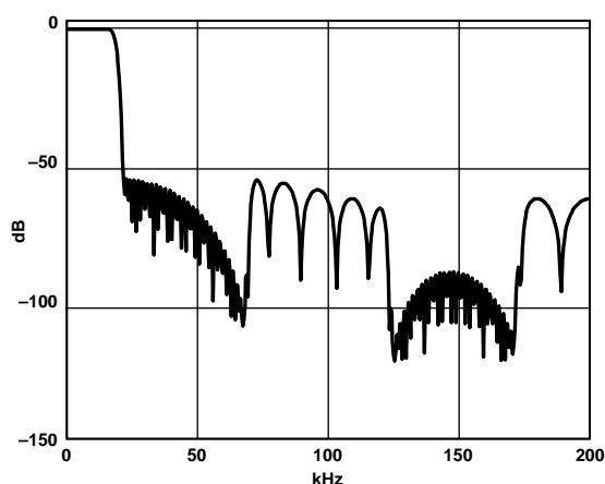
TPC 5. DAC Composite Filter Response, f_s = 48 \text{ kHz}
