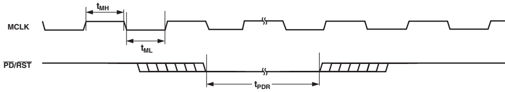
Figure 1. MCLK and RESET Timing
