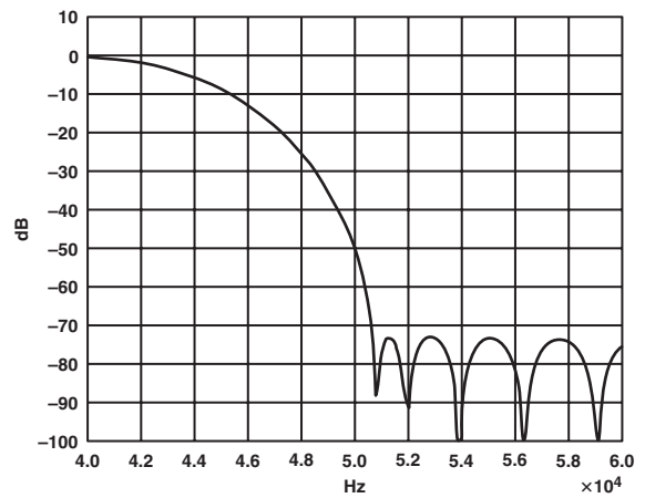
TPC 6. Transition Band Response, 4× Mode
