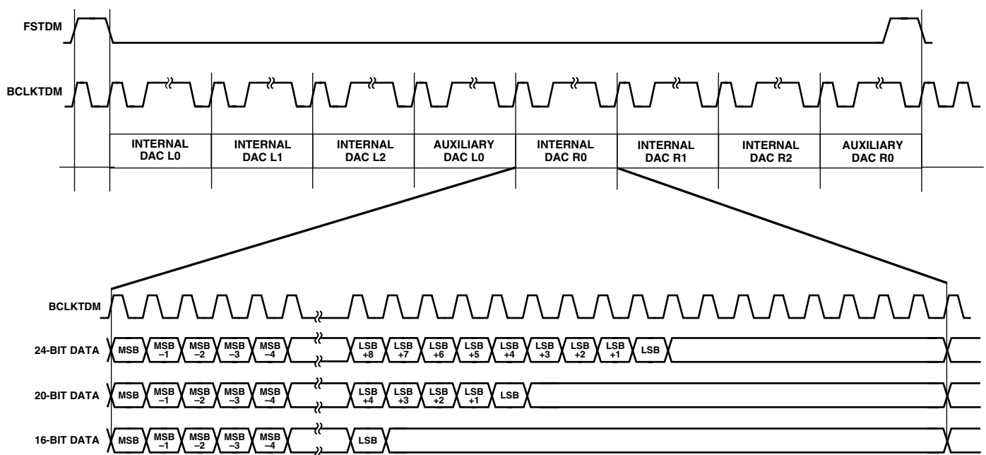
Figure 9. TDM Mode Timing
