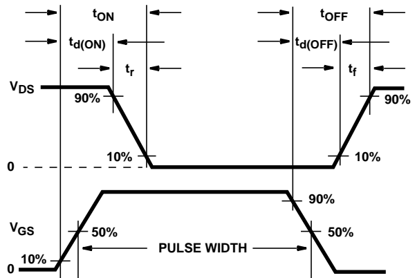
FIGURE 16. SWITCHING WAVEFORMS
