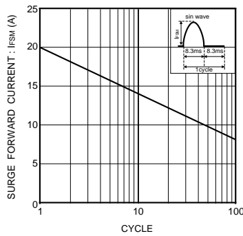
Fig.5 Forward peak surge current
