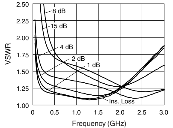
VSWR vs. Frequency (85°C)
