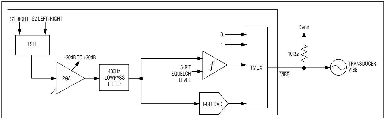
Figure 7. Transducer/Vibe Functional Diagram
