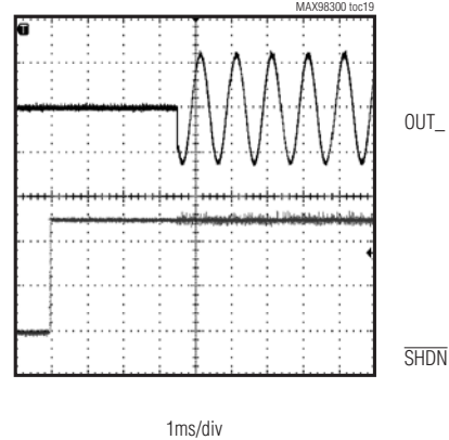
SHUTDOWN WAVEFORM
