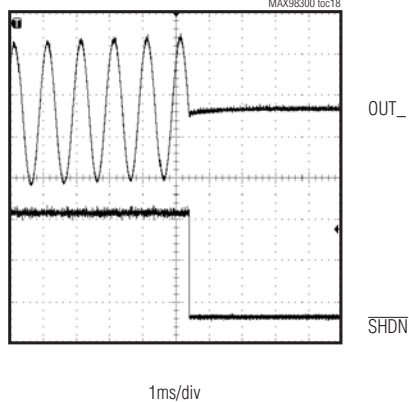
STARTUP WAVEFORM
