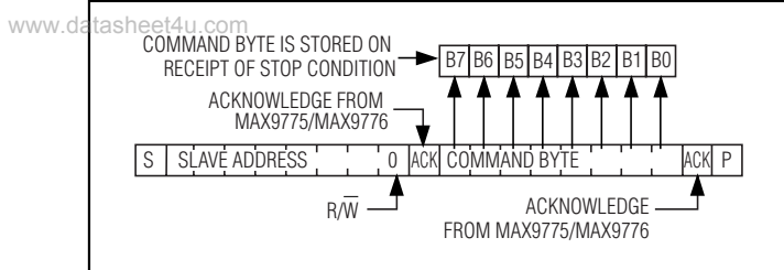
Figure 11. Write Data Format Example
