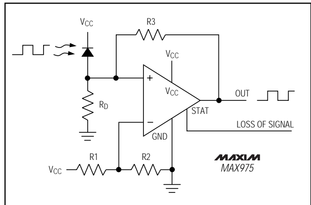
Figure 4. IR Receiver
