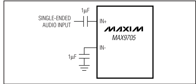
Figure 5. Single-Ended Input
