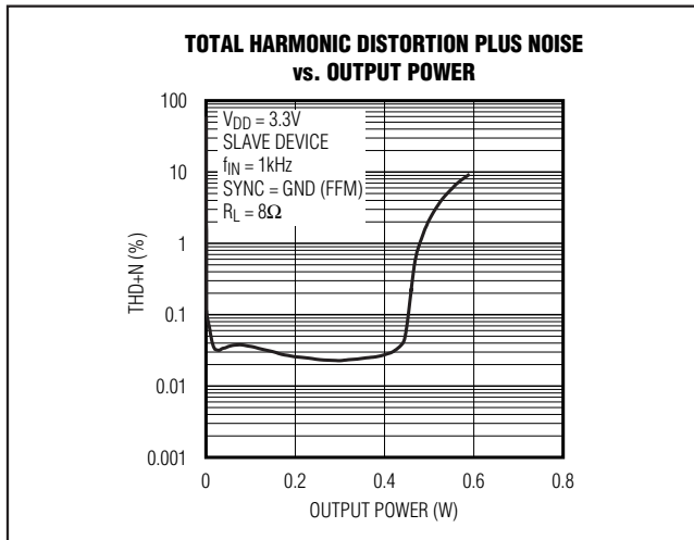
Figure 7. Master-Slave THD+N
