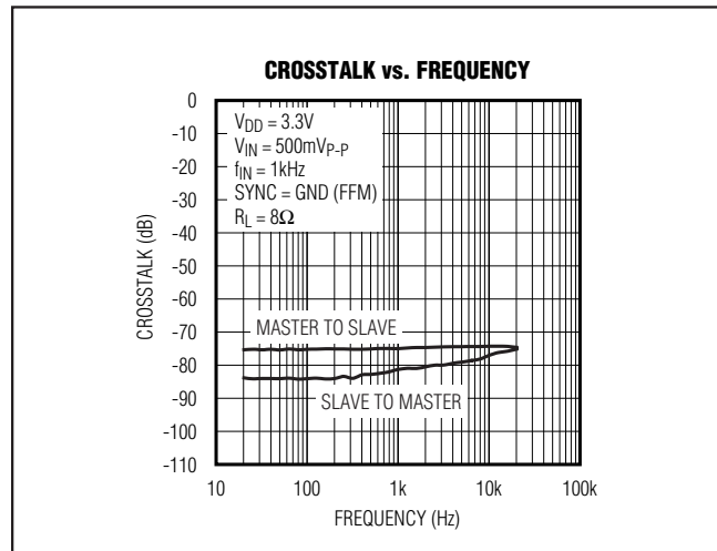
Figure 8. Master-Slave Crosstalk
