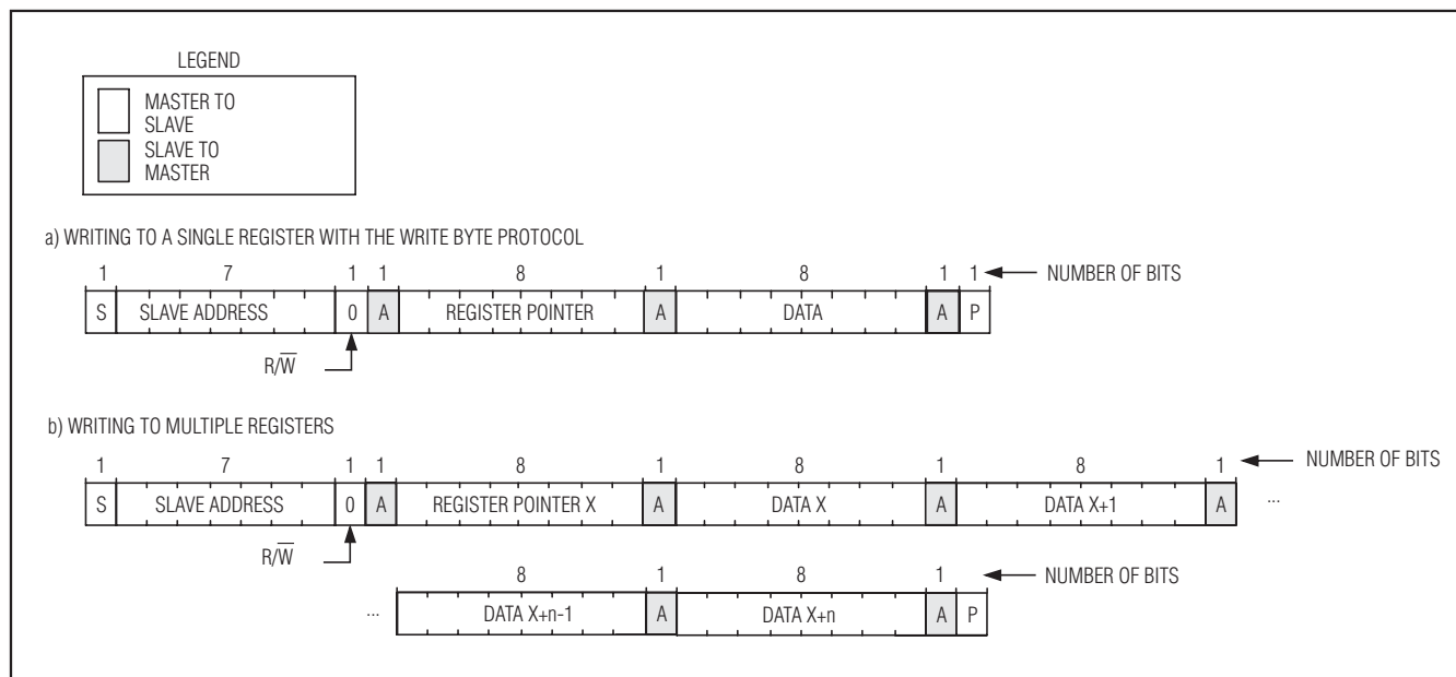
Figures 14a and 14b. Writing to the MAX8649
