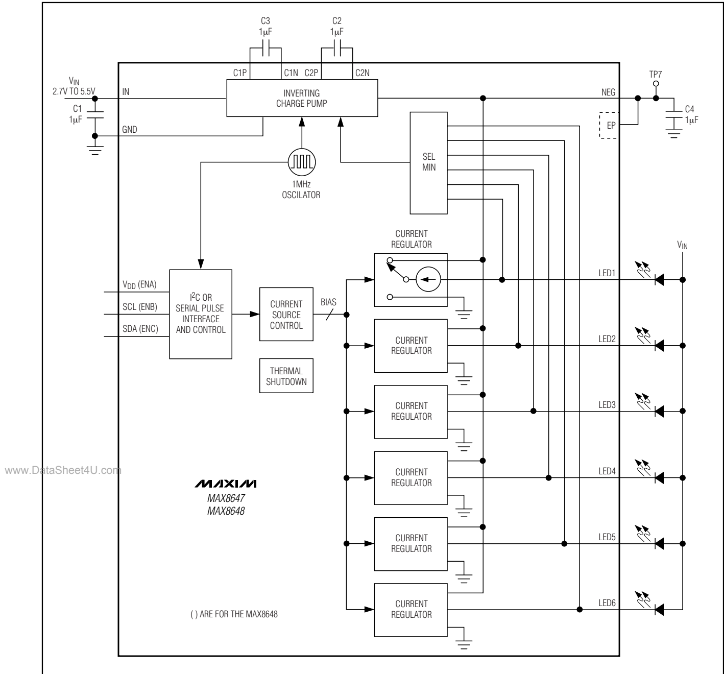
Figure 1. Block Diagram and Application Circuit
