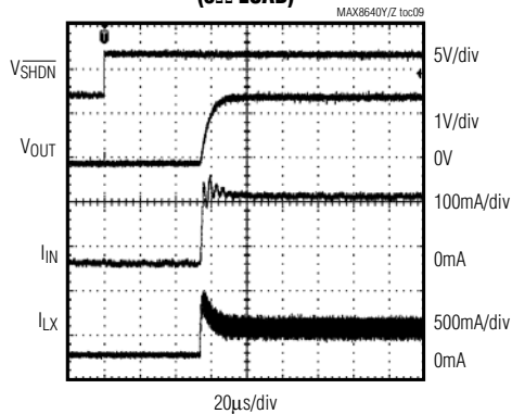
HEAVY-LOAD STARTUP WAVEFORM (5Ω LOAD)
