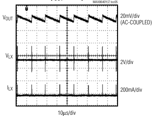
LIGHT-LOAD SWITCHING WAVEFORMS ( I_{OUT} = 1mA )
