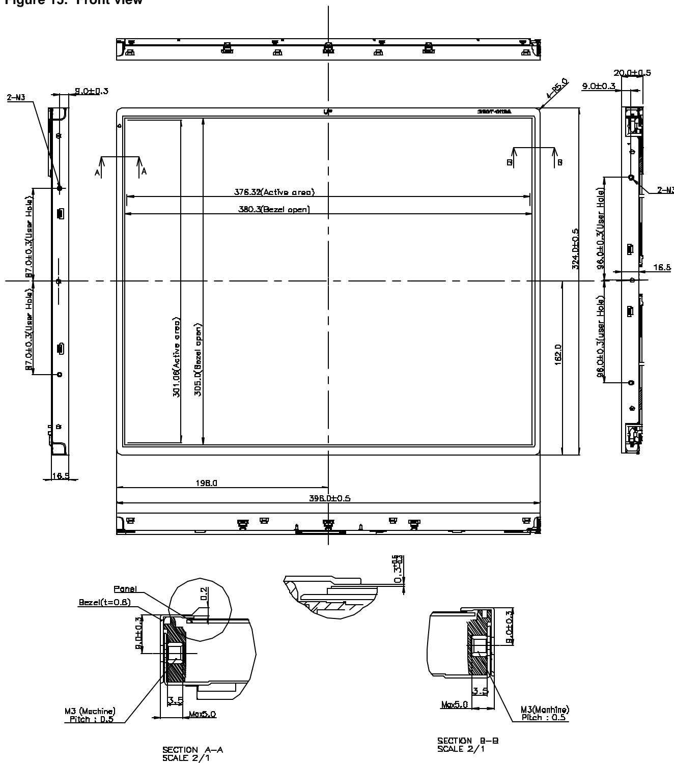
Figure 15. Front view
