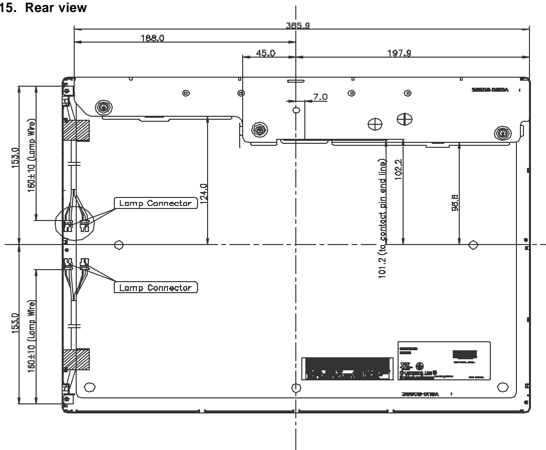
Figure 15. Rear view
