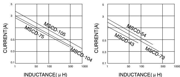
Typical Electrical Characteristics
