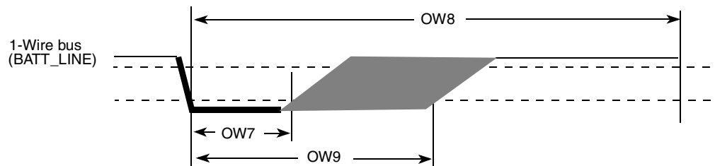
Figure 64. Read Sequence Timing Diagram
