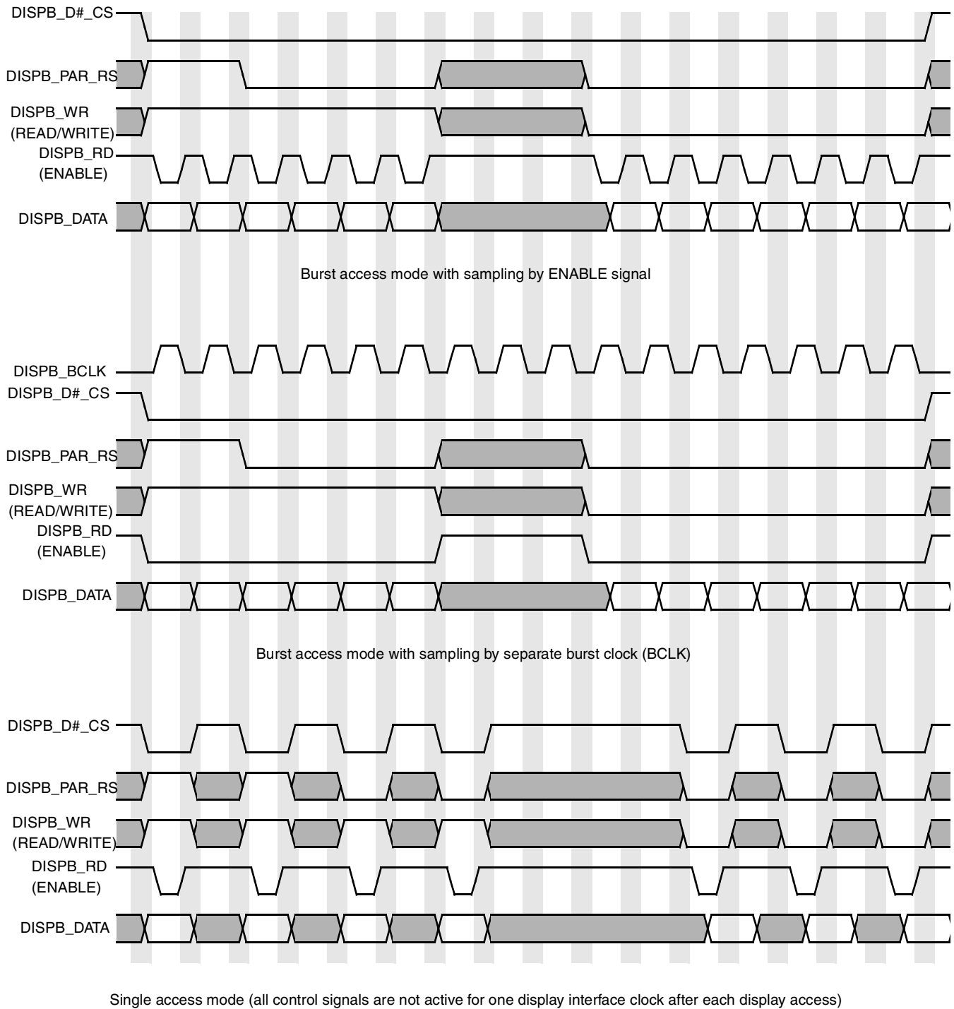
Figure 45. Asynchronous Parallel System 68k Interface (Type 2) Burst Mode Timing Diagram
