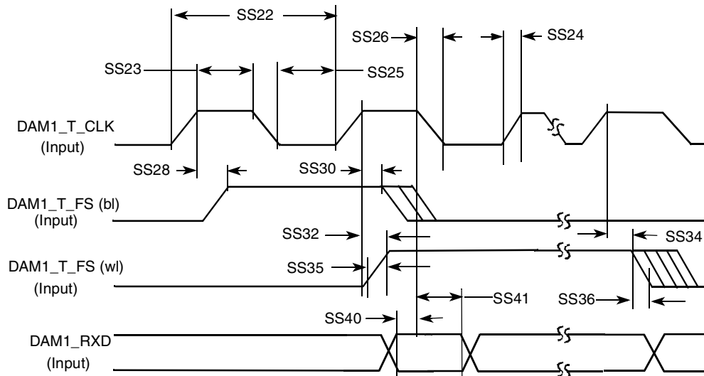
Figure 86. SSI Receiver with External Clock Timing Diagram
