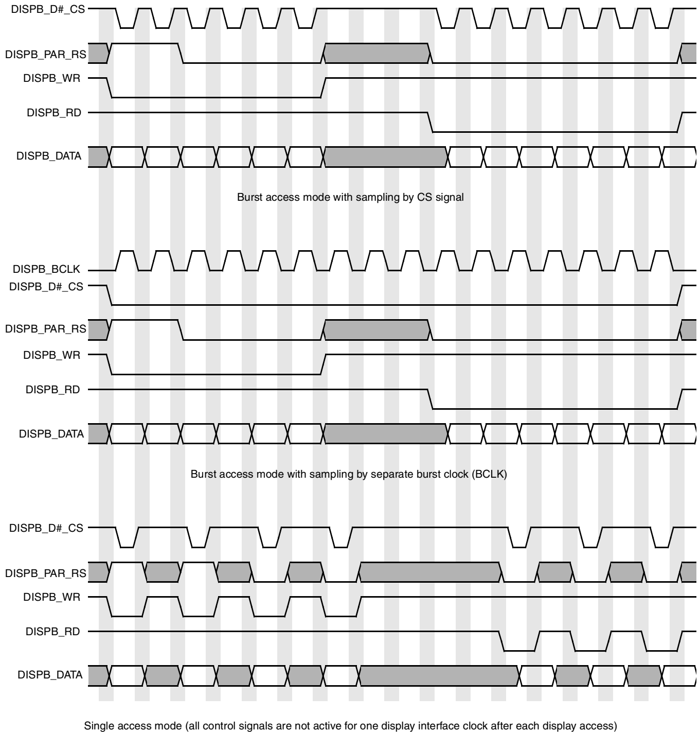
Figure 42. Asynchronous Parallel System 80 Interface (Type 1) Burst Mode Timing Diagram
