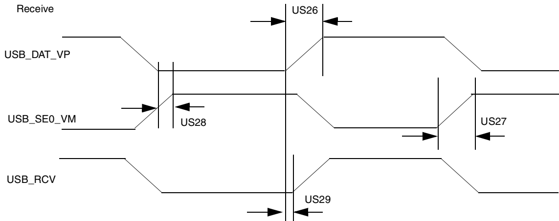
Figure 96. USB Receive Waveform in VP_VM Bidirectional Mode
