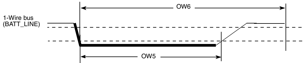
Figure 62. Write 0 Sequence Timing Diagram
