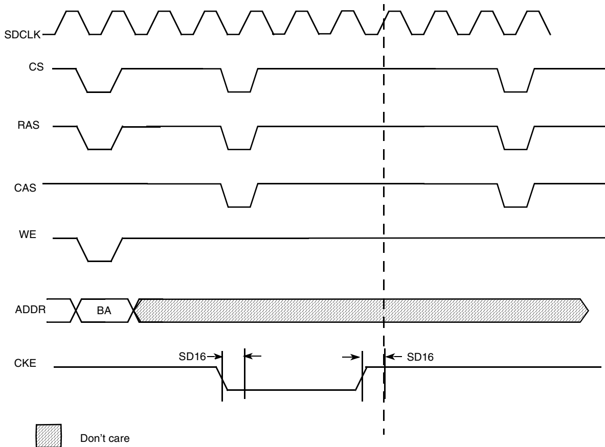
Figure 22. SDRAM Self-Refresh Cycle Timing Diagram
