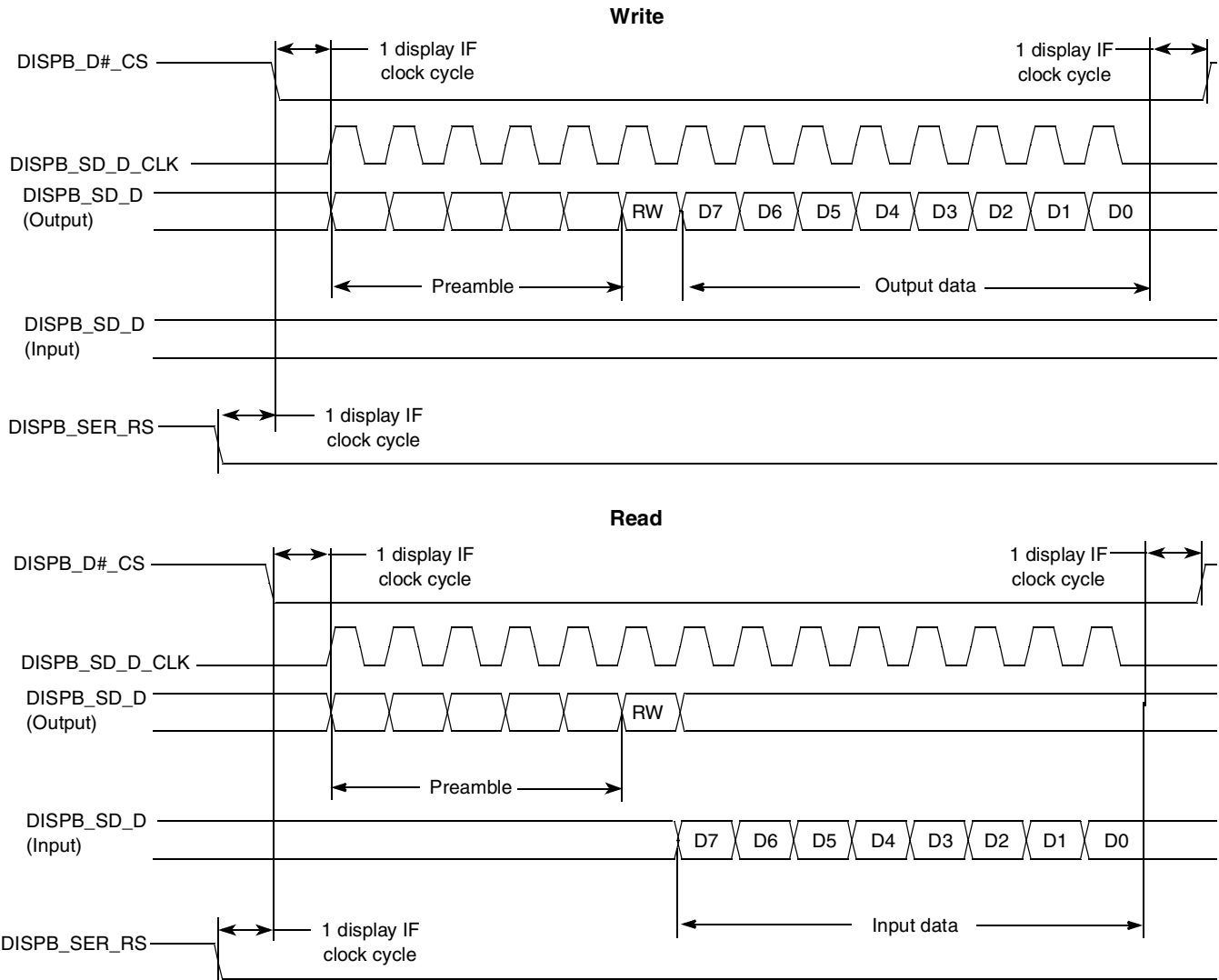
Figure 54. 5-Wire Serial Interface (Type 2) Timing Diagram
