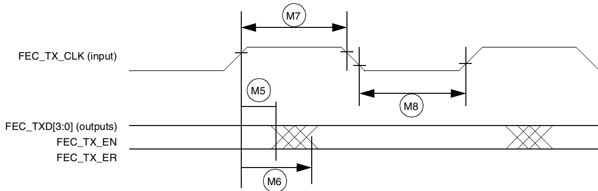
Figure 29. MII Transmit Signal Timing Diagram
