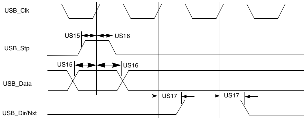
Figure 76. USB Transmit/Receive Waveform in Parallel Mode
