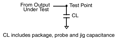
Figure 2. Load Circuit for Output Pad
