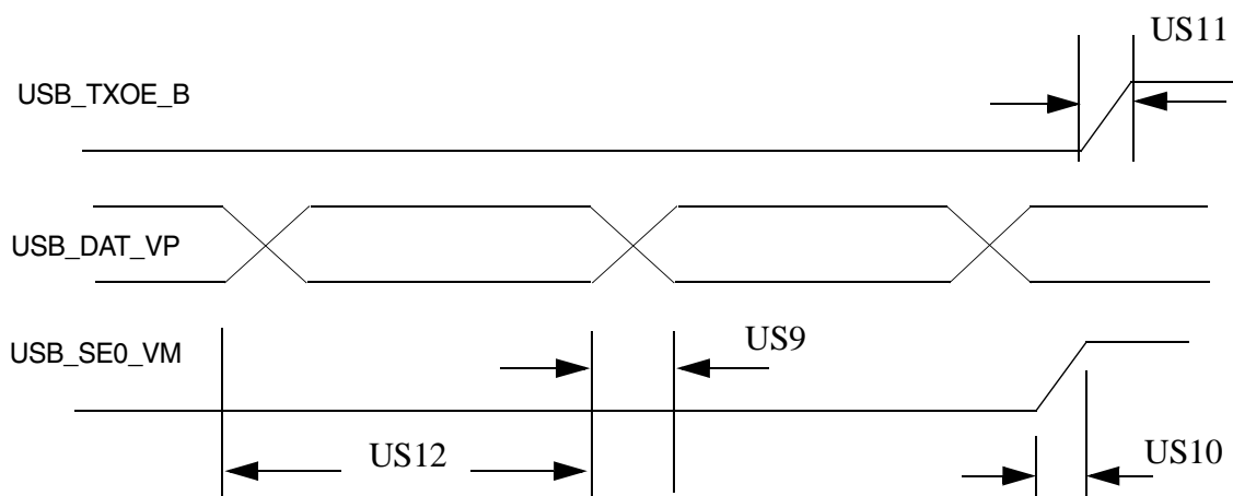
Figure 93. USB Transmit Waveform in DAT_SE0 Unidirectional Mode
