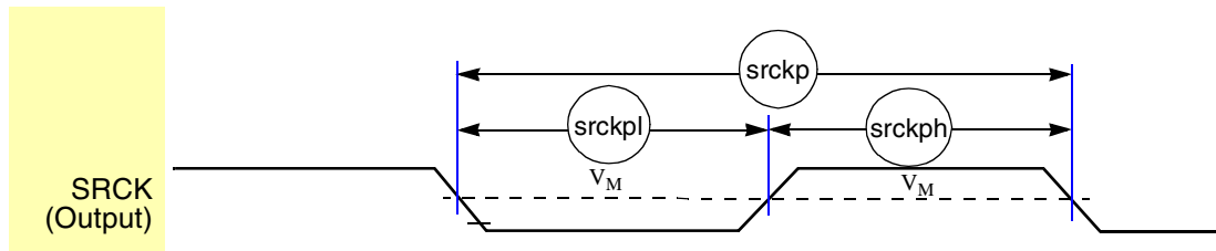
Figure 81. SRCK Timing
