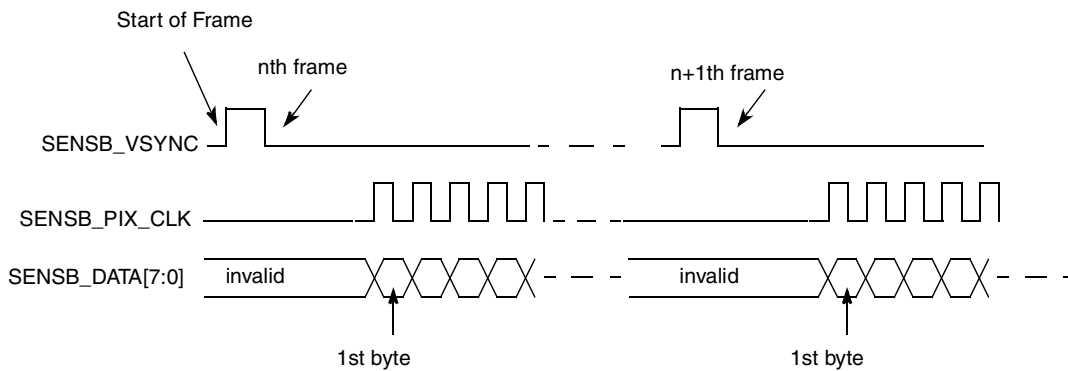
Figure 34. Non-Gated Clock Mode Timing Diagram
