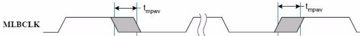
Figure 60. MediaLB Pulse Width Variation Timing
