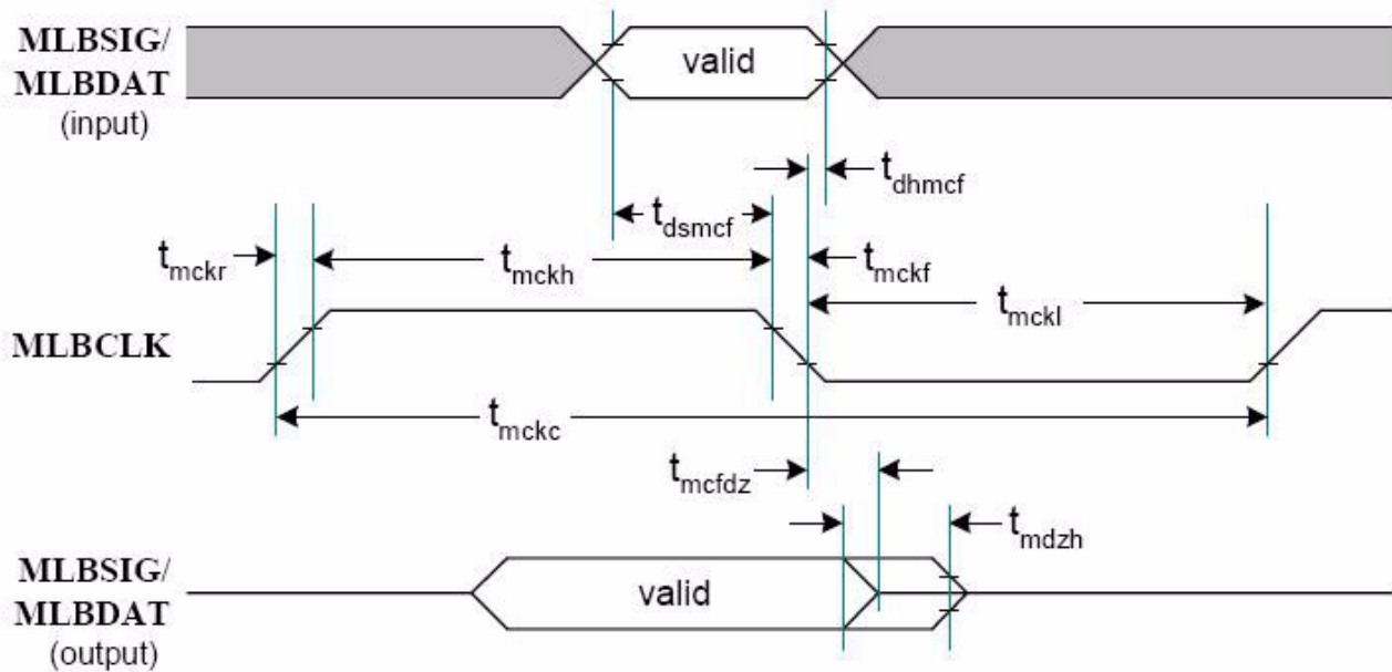
Figure 59. MediaLB Timing
