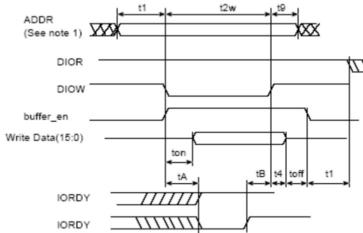
Figure 67. PIO Write Timing Diagram
