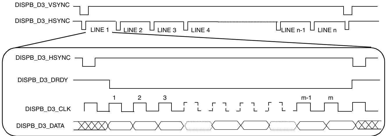
Figure 36. Interface Timing Diagram for TFT (Active Matrix) Panels
