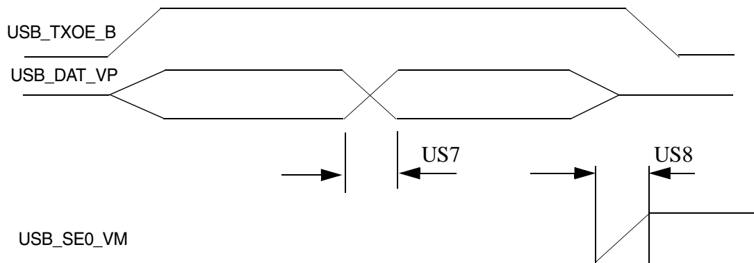
Figure 92. USB Receive Waveform in DAT_SE0 Bidirectional Mode
