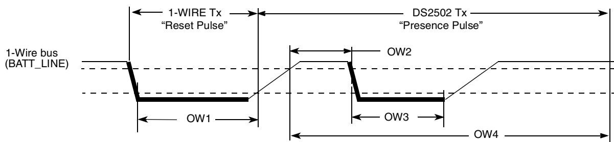
Figure 61. Reset and Presence Pulses (RPP) Timing Diagram
