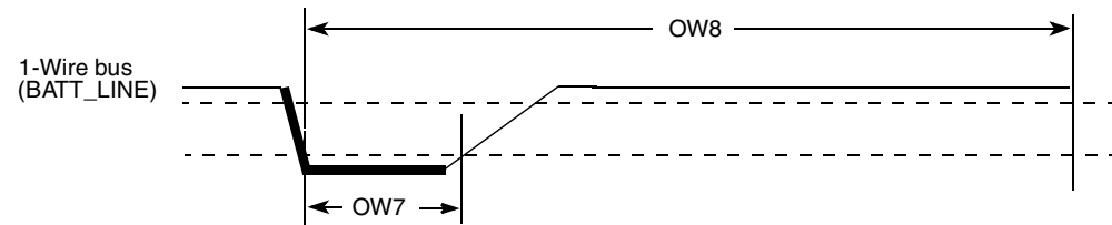
Figure 63. Write 1 Sequence Timing Diagram
