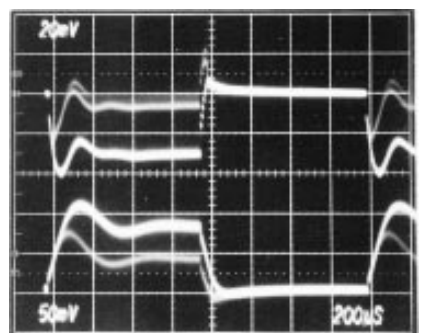
LOAD-TRANSIENT RESPONSE
